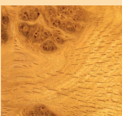
Eiche Cluster
